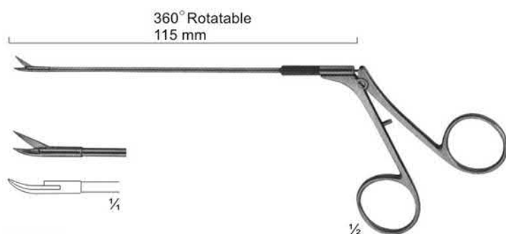
02-3019 CASPAR Micro Scissor Curved
